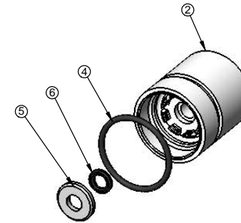
10598 END PLUG ASSY
