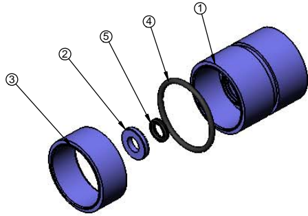
10598-02 END PLUG ASSY,2750, NHWP,DF
